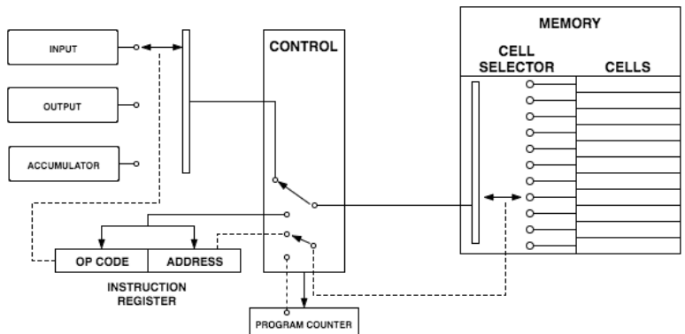
Fig. No. 12. Instruction register reading a word into the memory.
