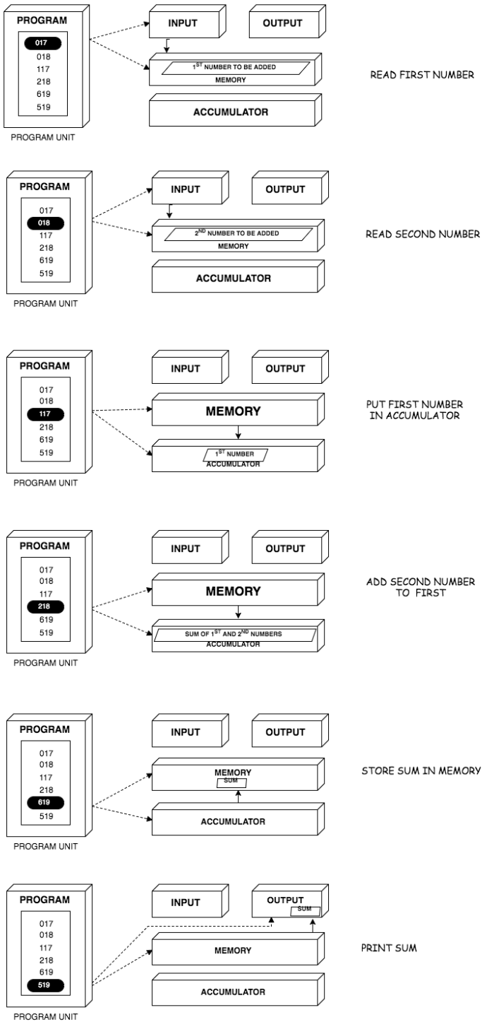
Fig. No.8. SIMCO adding two numbers.
