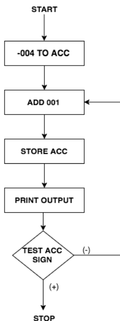
Fig. No. 15. Flow chart of rocket—launching countdown.
