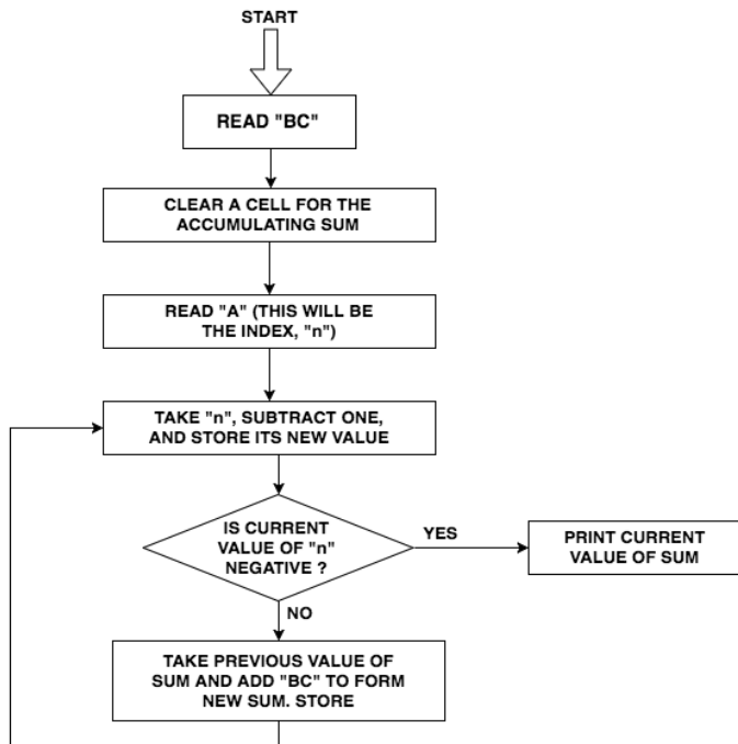
Fig. No. 16. Flow chart of single—digit multiplication.
