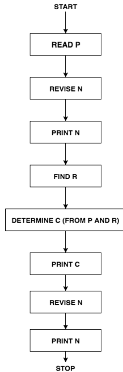
Fig. No. 18. Macro flow chart for improved Nim game.
