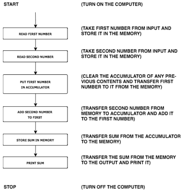
Fig. No. 7. Flow chart for addition with SIMCO.
