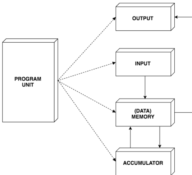
Fig. No. 1. Block diagram for SIMCO.
