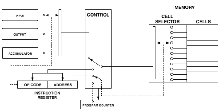
Fig. No. 10. Control adding 1 to the program counter.
