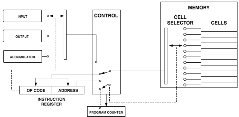
Fig. No. 11. Control fetching a word to the instruction register.
