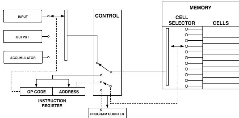
Fig. No. 9. Stored-program computer.
